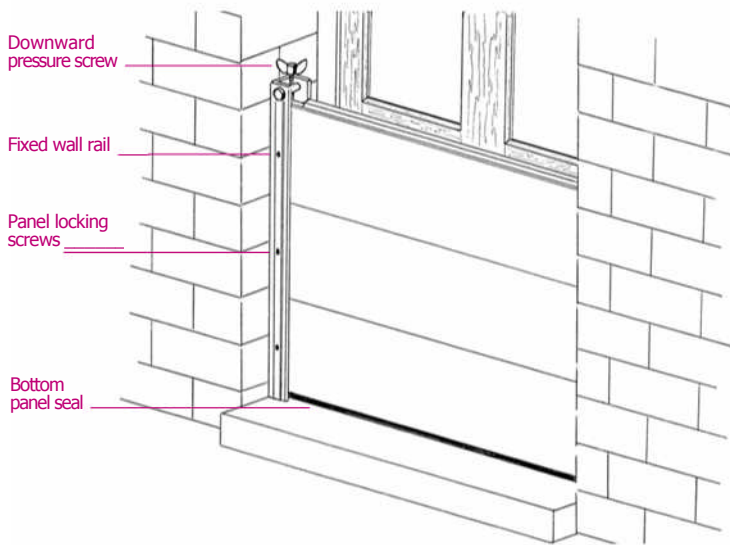
Wall fixture side view
